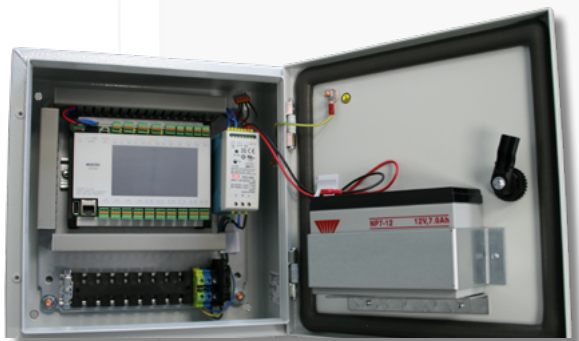
Steel wall casing, open
