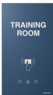
Access reader with glass plate in desired colour (RAL), room designation, DND, MUR and bell
